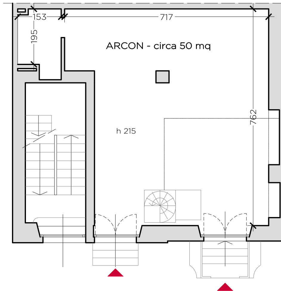
PIANO TERRA
